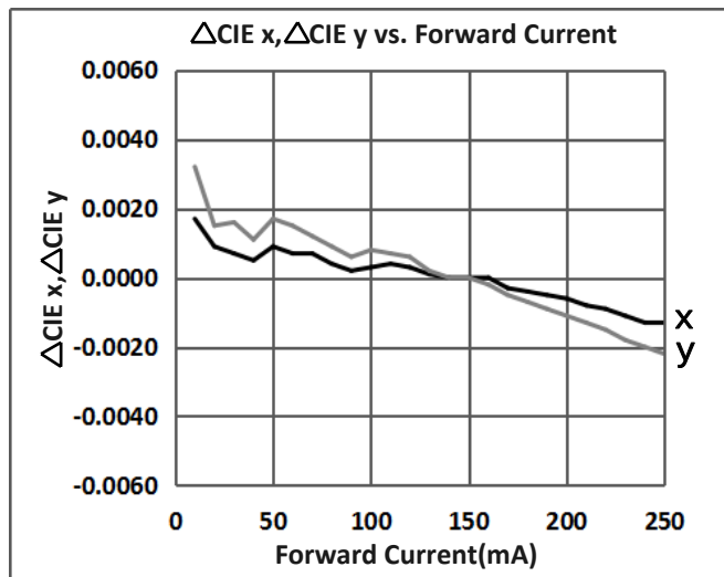
d) Color Shift Characteristics, T_s = 25^\circ\text{C} , I_f = 150\text{ mA}
